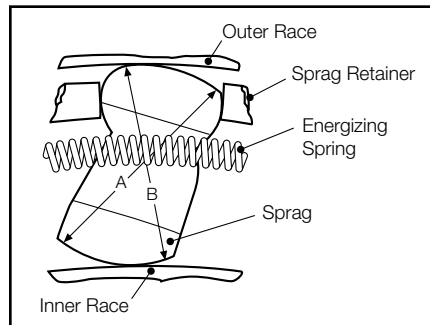
Figure 1 Detail of sprag. Dimension "A" is greater than dimension "B."
